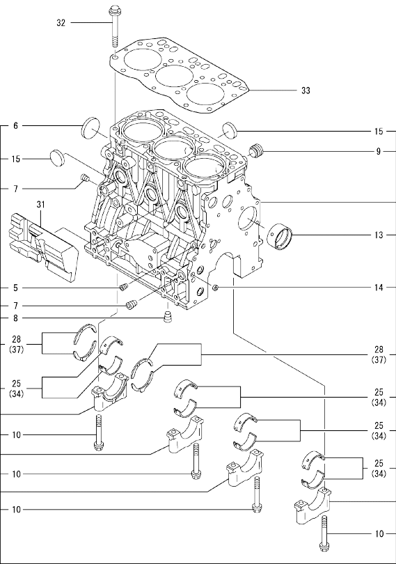
Fig.1. CYLINDER BLOCK
