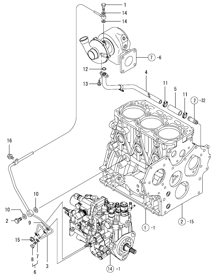
Fig.10. LUB.OIL LINE
