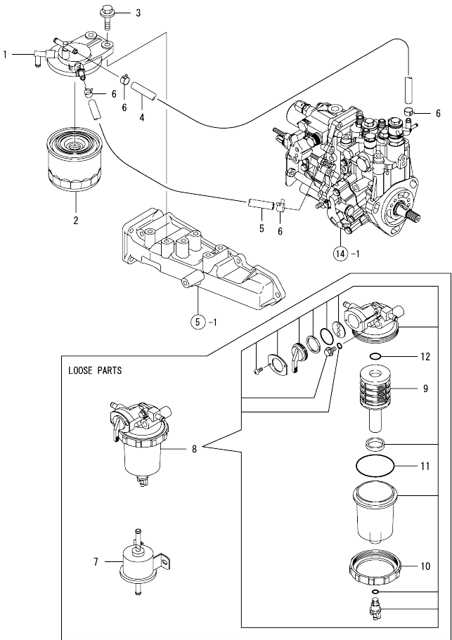
Fig.17. FUEL LINE
